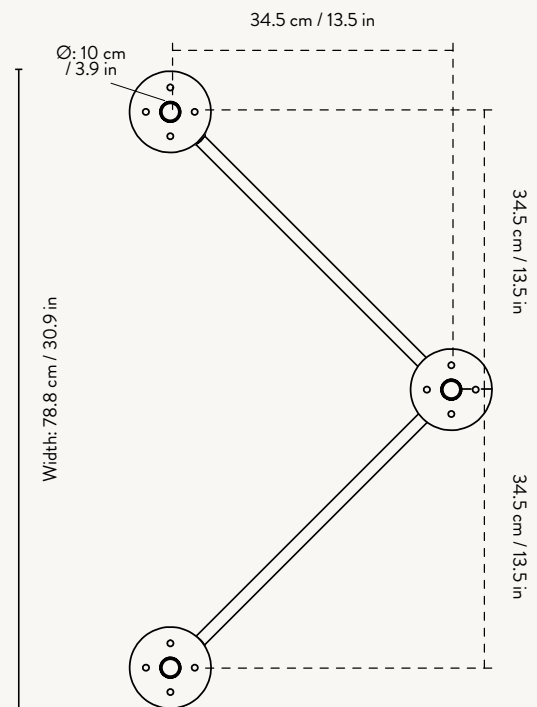
MINGLE TABLE LEGS - W68 TOP VIEW
